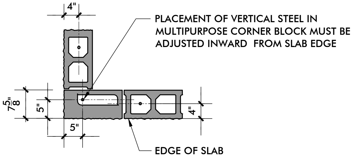
MULTIPURPOSE CORNER UNIT - 8"
