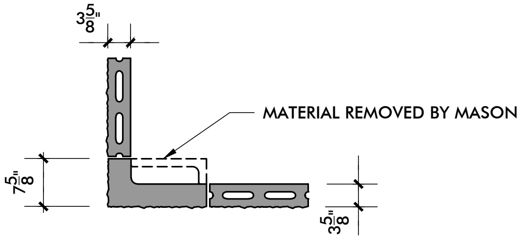
MULTIPURPOSE CORNER UNIT - 4"
