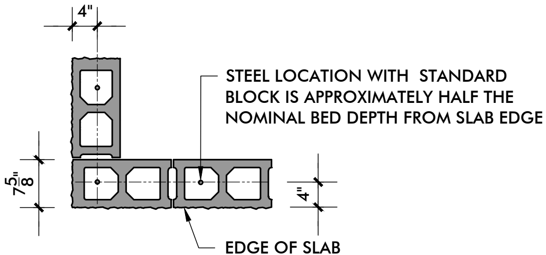
STANDARD CORNER UNIT
